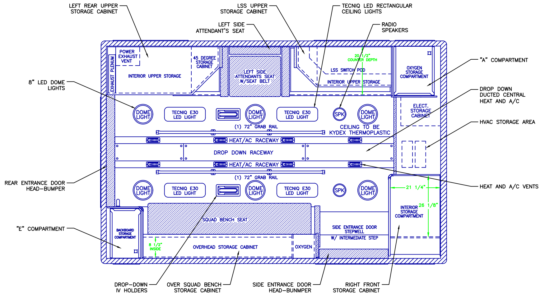
CEILING VIEW
