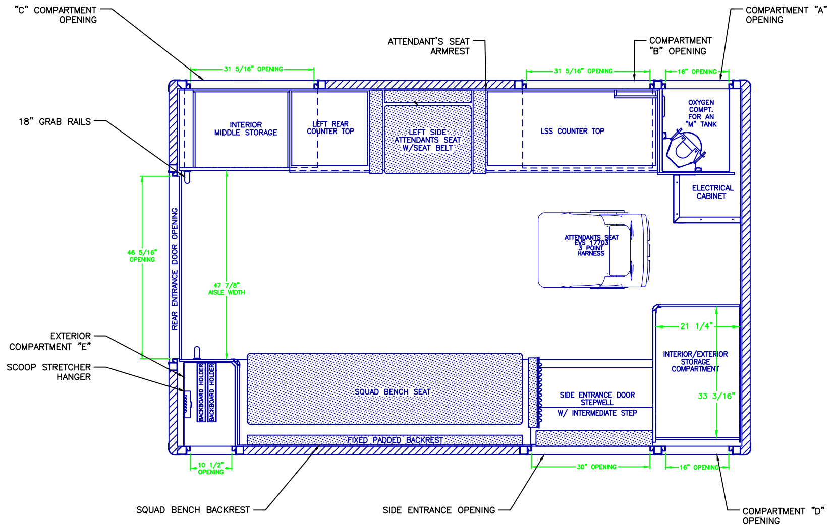
FLOOR PLAN
