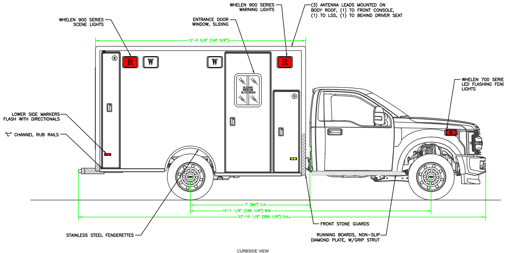
CURBSIDE VIEW
