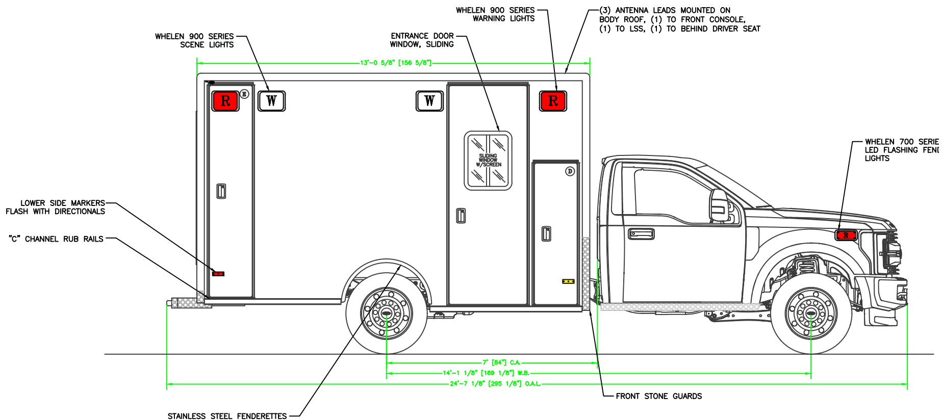
CURBSIDE VIEW
