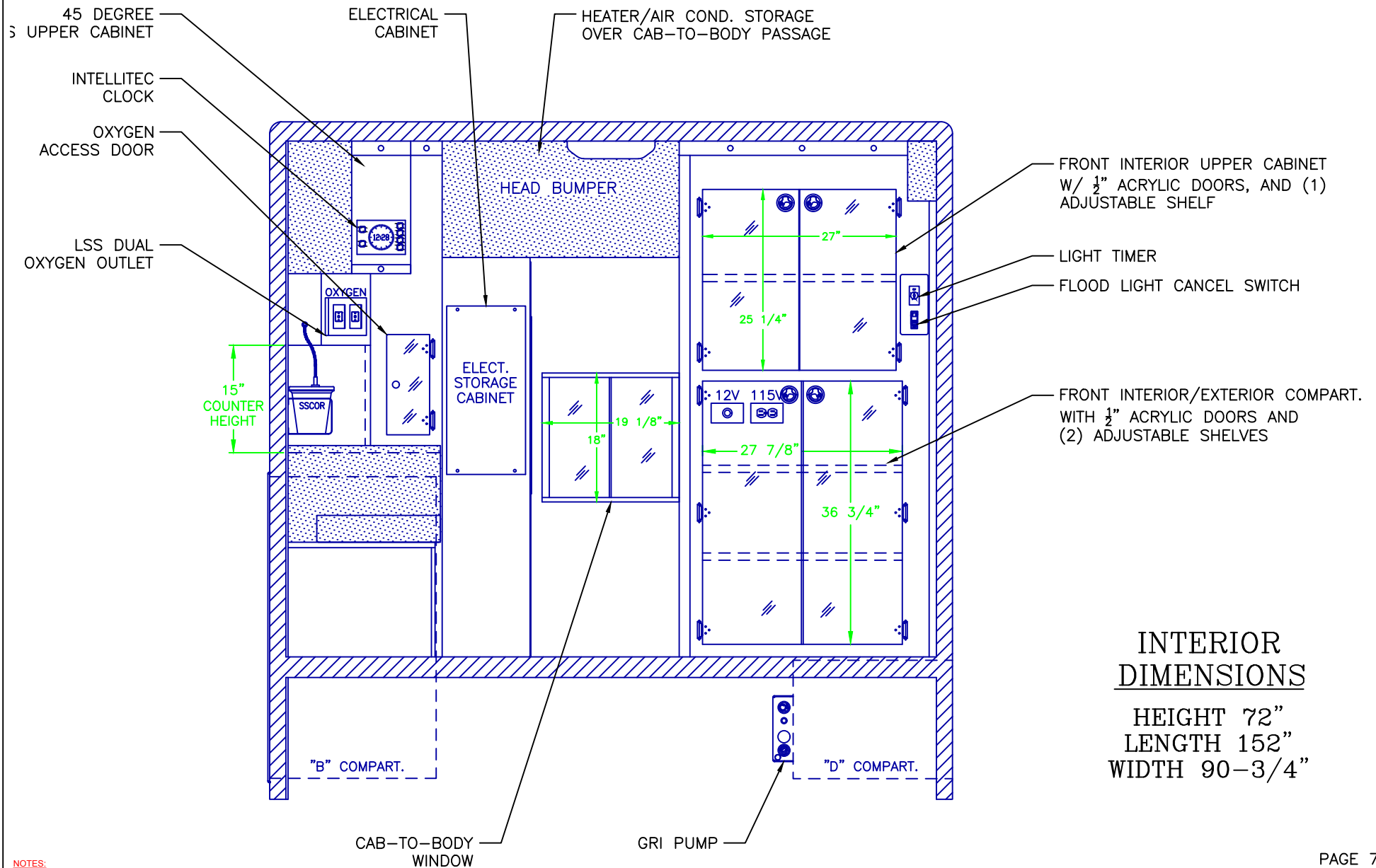
FRONT VIEW
